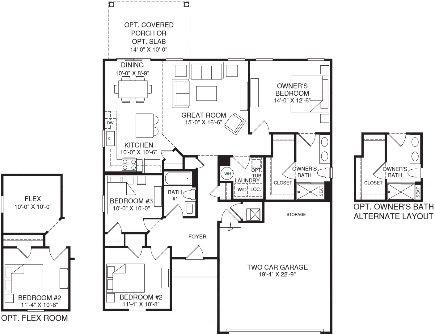
MAIN LEVEL
