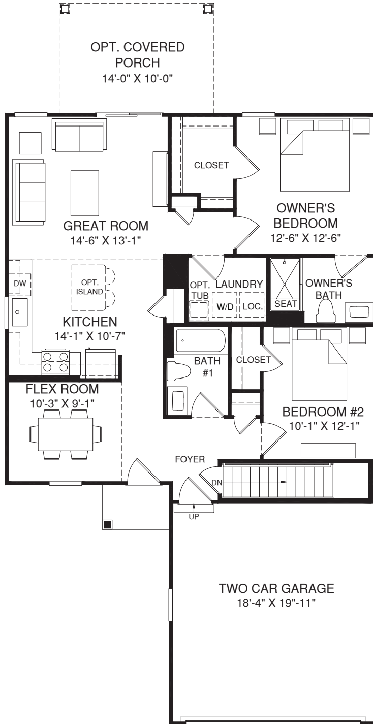
MAIN LEVEL
