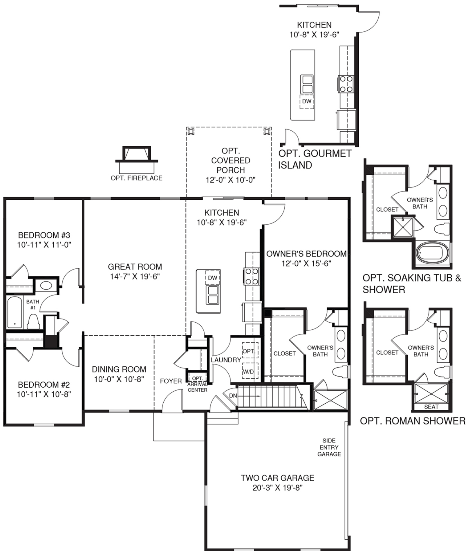
MAIN LEVEL
