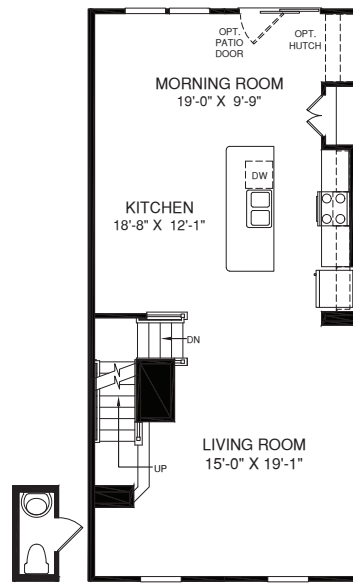
MAIN LEVEL
