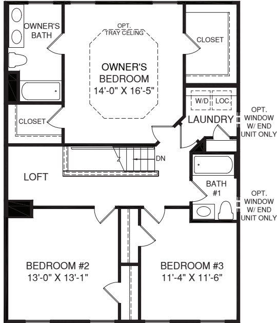
UPPER LEVEL
