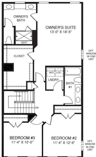
UPPER LEVEL
