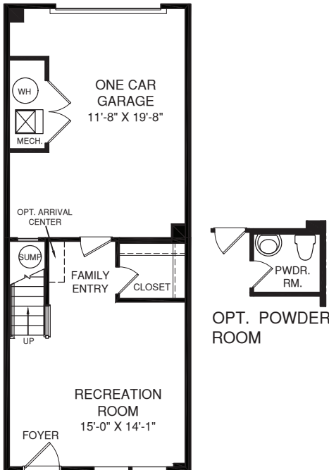
ONE CAR GARAGE W/ OPT. REC. ROOM
