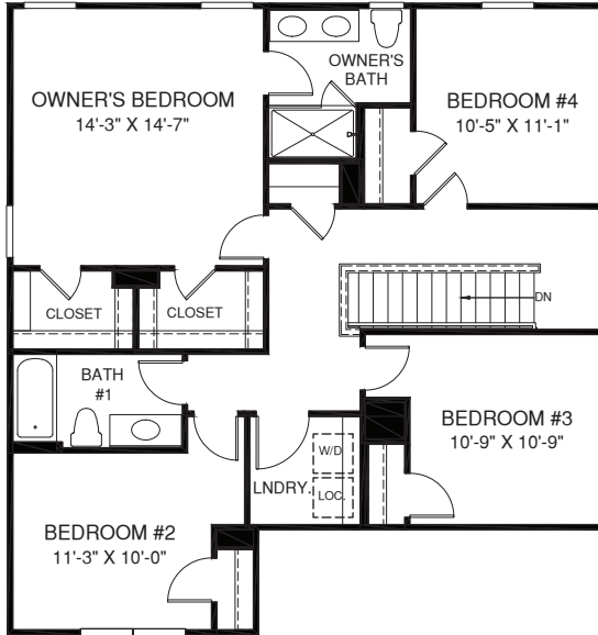
UPPER LEVEL
