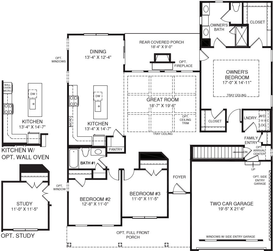
MAIN LEVEL
