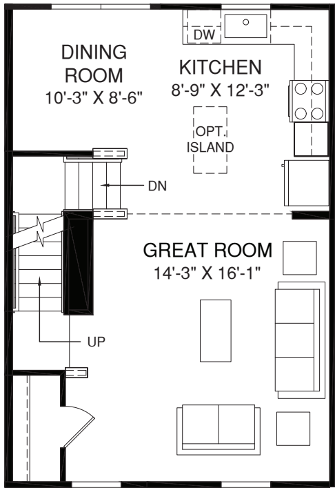
MAIN LEVEL
