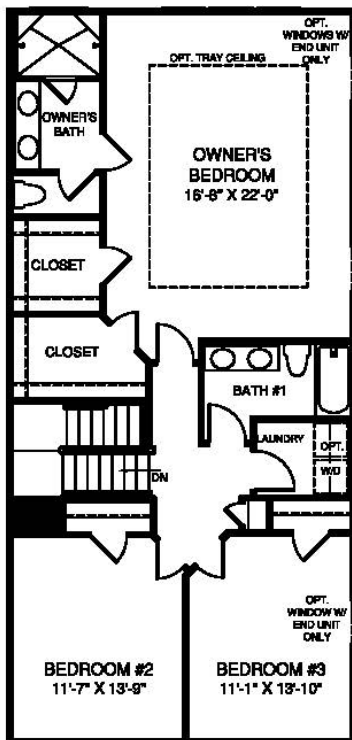
THREE BEDROOM PLAN W/ 10' EXT. TO HOUSE
