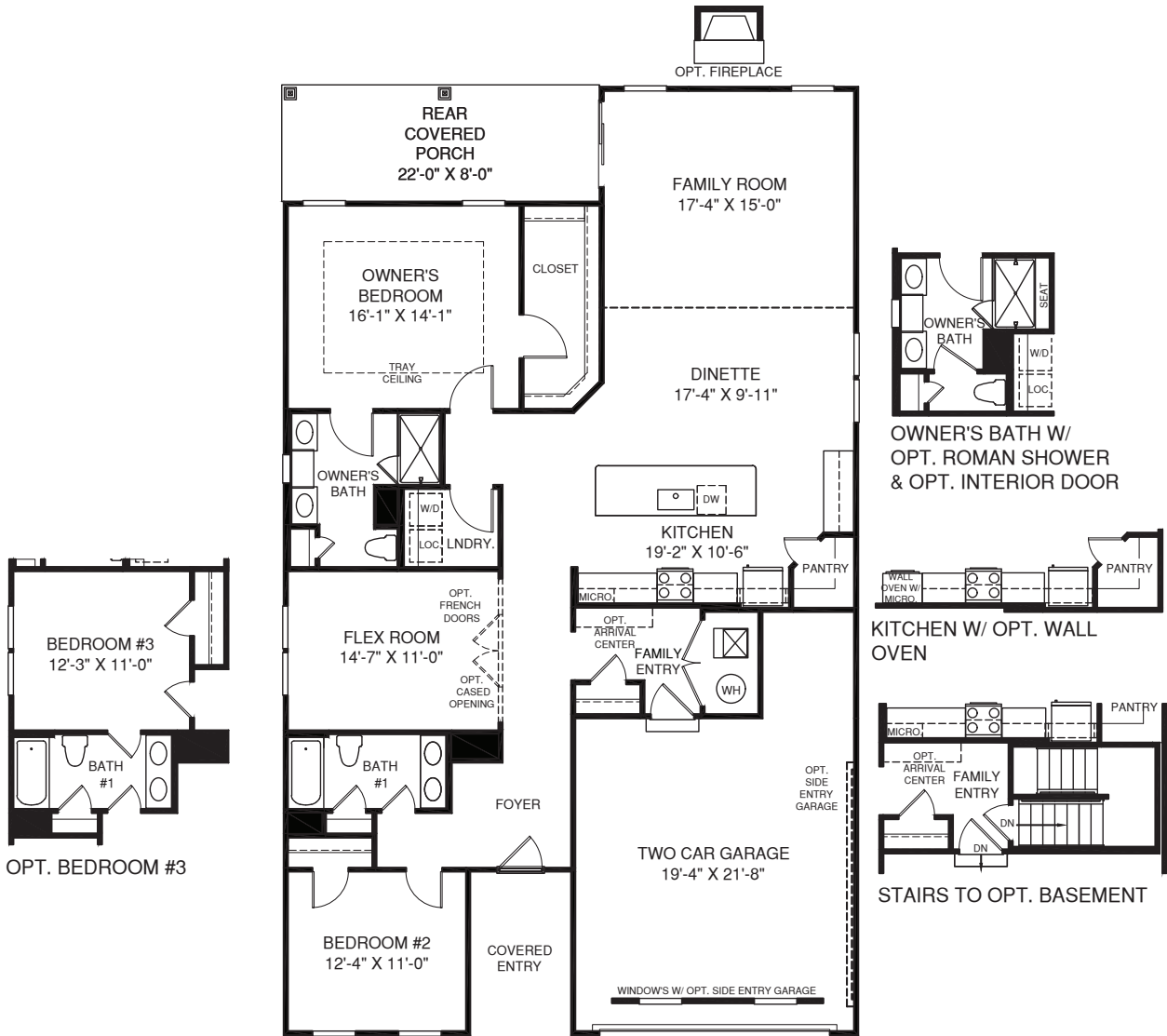
MAIN LEVEL
