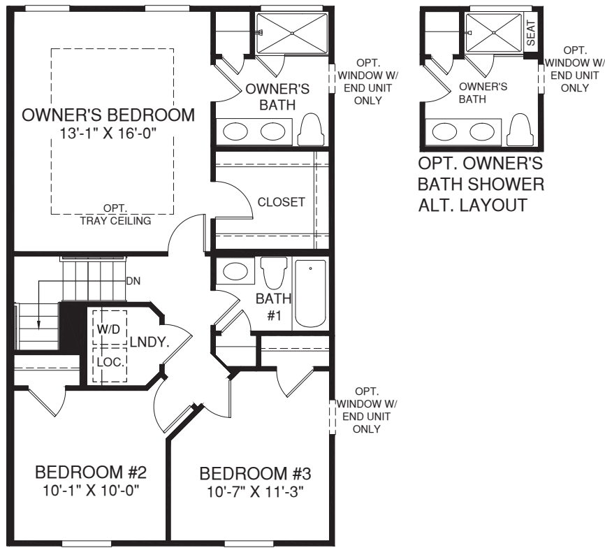
UPPER LEVEL
