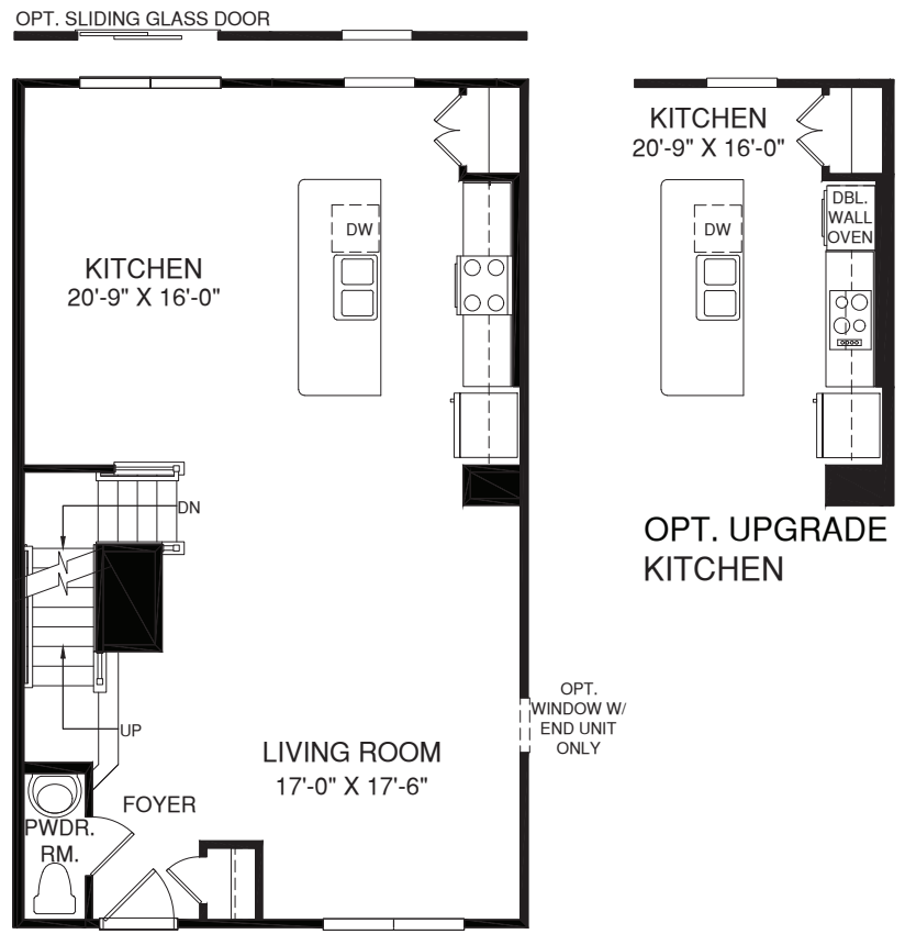
MAIN LEVEL
