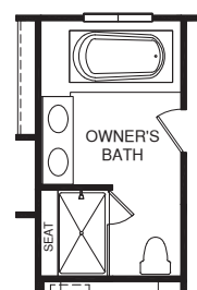
OPT. OWNER'S BATH W/ SOAKING TUB & SHOWER
