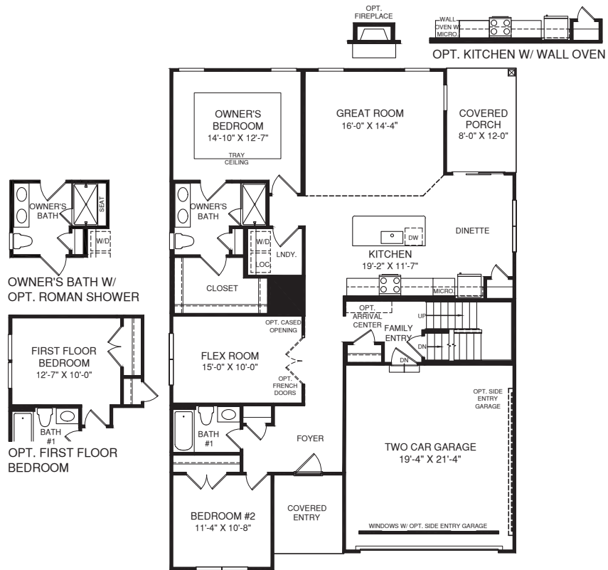
MAIN LEVEL
