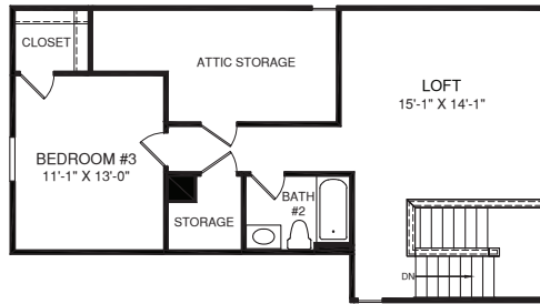
UPPER LEVEL
