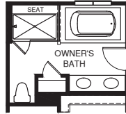
OPT. OWNER'S BATH W/ SOAKING TUB & SHOWER
