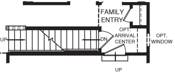
STAIRS W/ OPT. BONUS BEDROOM
