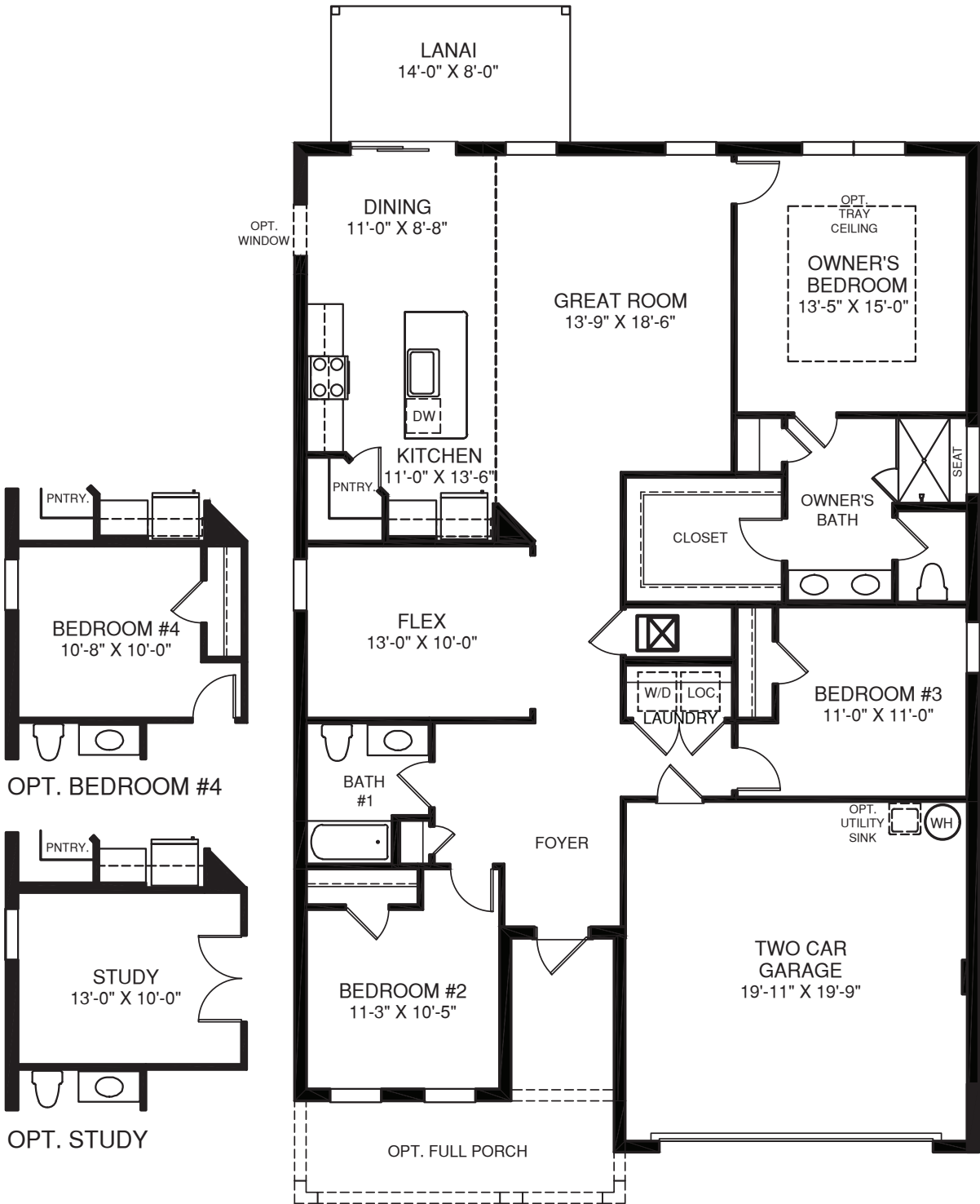
MAIN LEVEL
