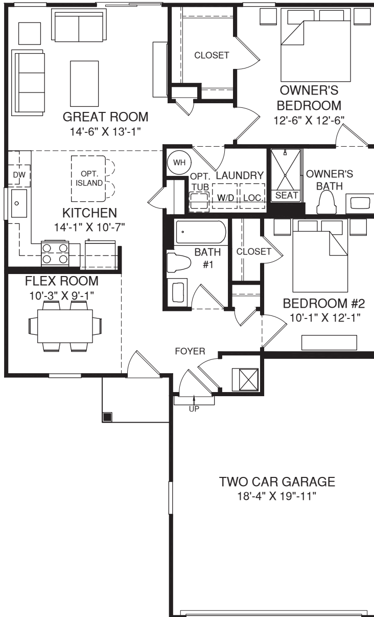
MAIN LEVEL
