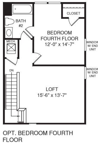
OPT. FOURTH FLOOR
