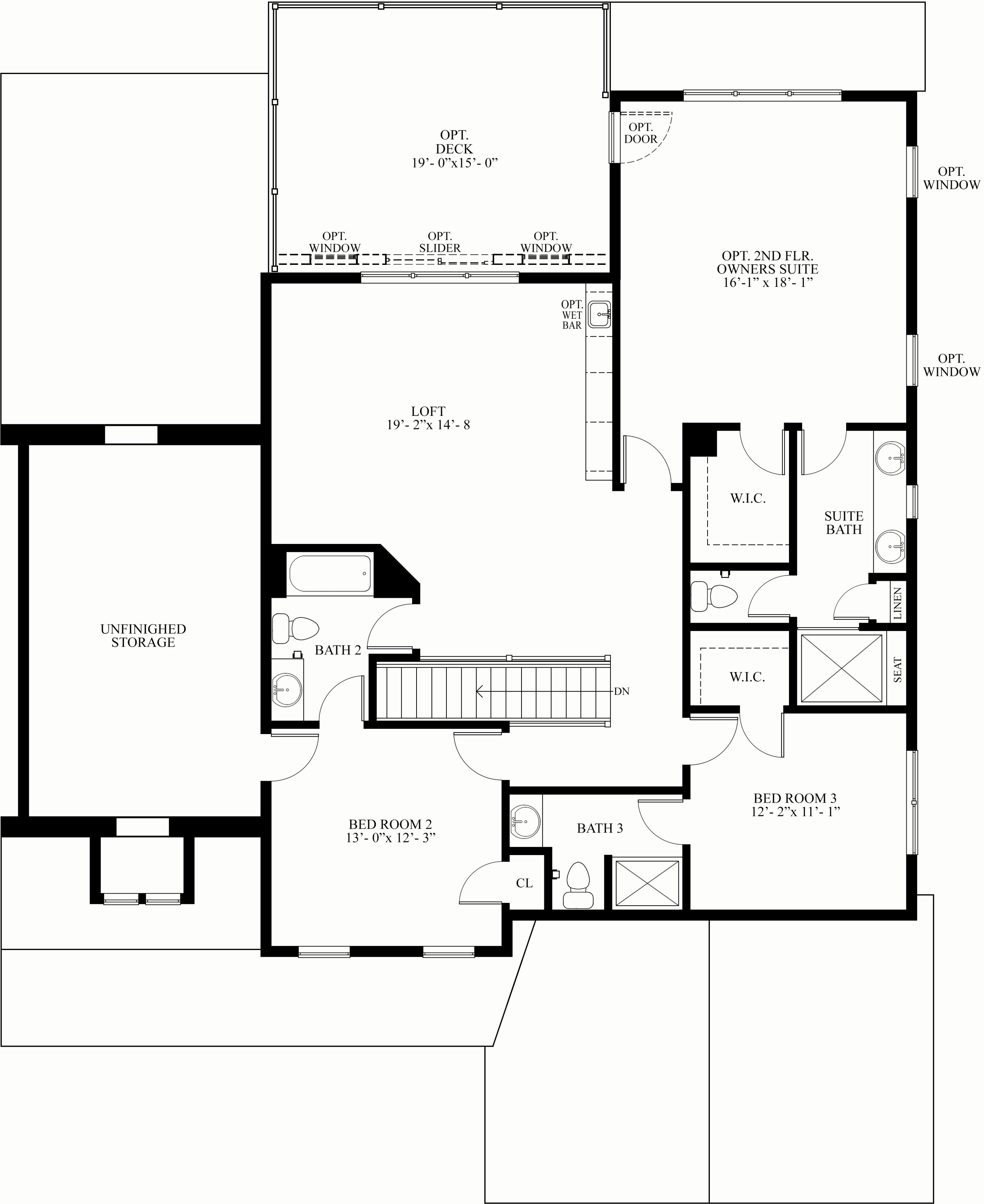
SECOND FLOOR PLAN EL A, EL B DUAL OWNER’S SUITE MSS. CRAWL SP
