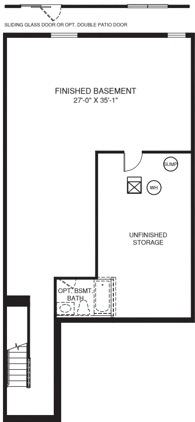
LOWER LEVEL
