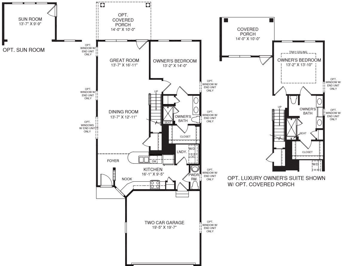
MAIN LEVEL
