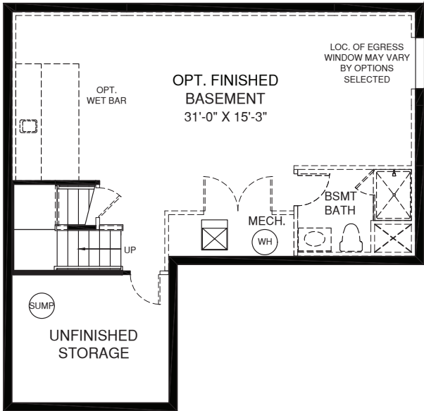
LOWER LEVEL
