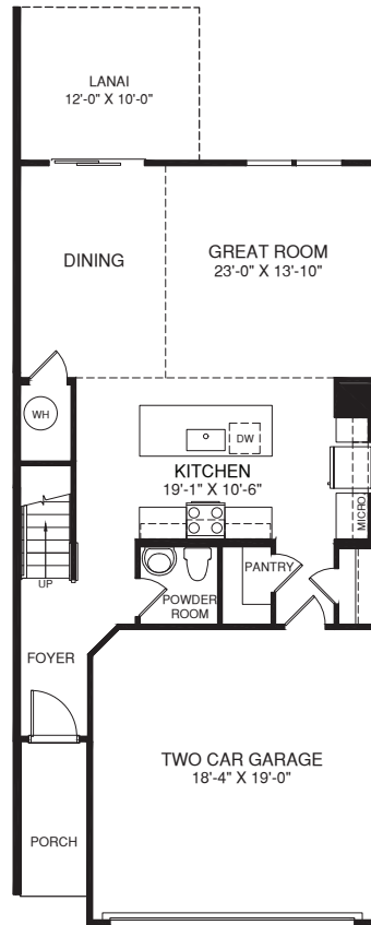
MAIN LEVEL
