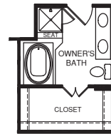
OPT. OWNER'S BATH W/ SOAKING TUB & SHOWER
