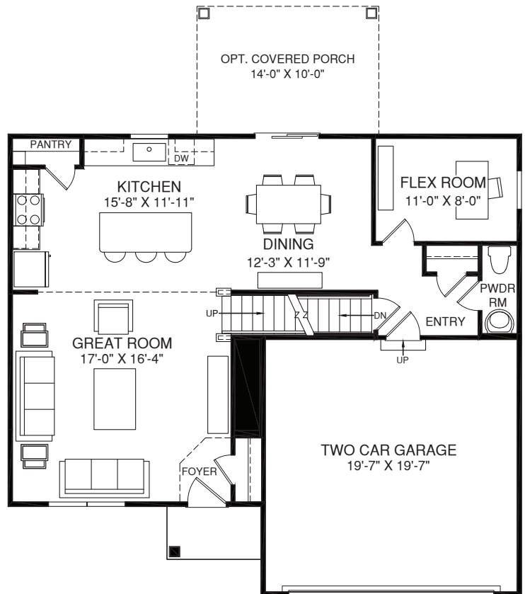
MAIN LEVEL
