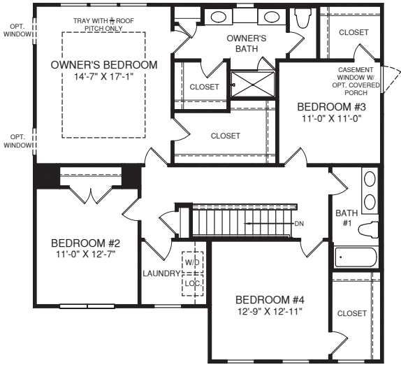
UPPER LEVEL
