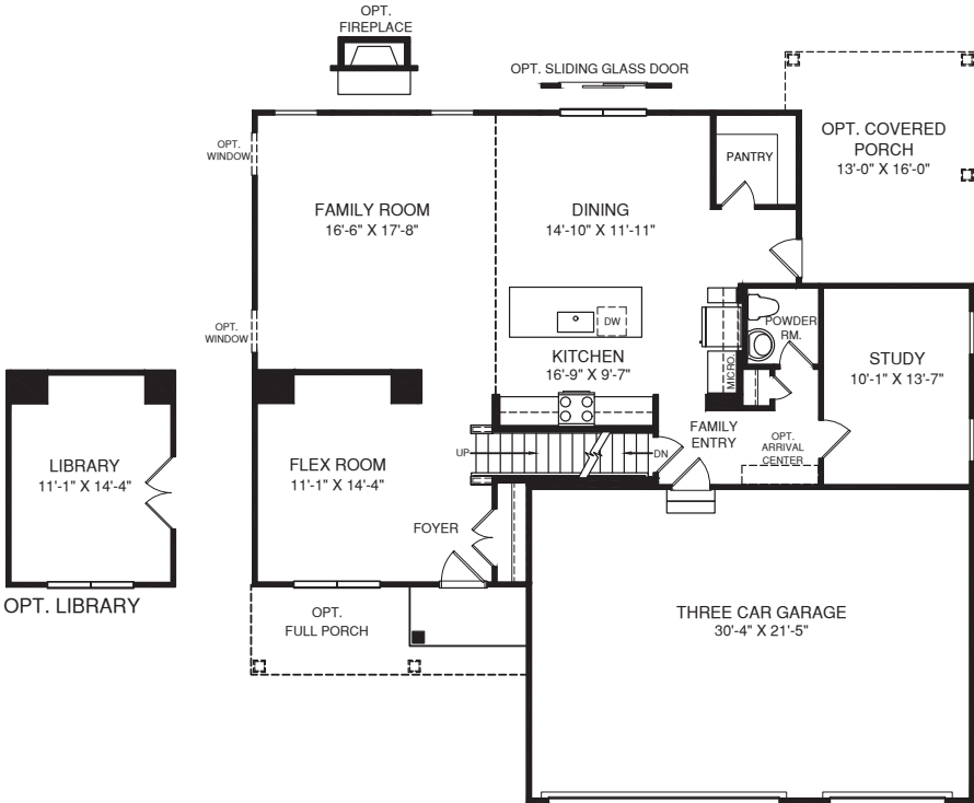
MAIN LEVEL
