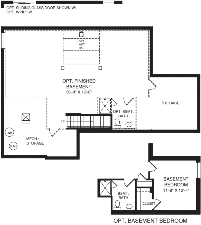
LOWER LEVEL
