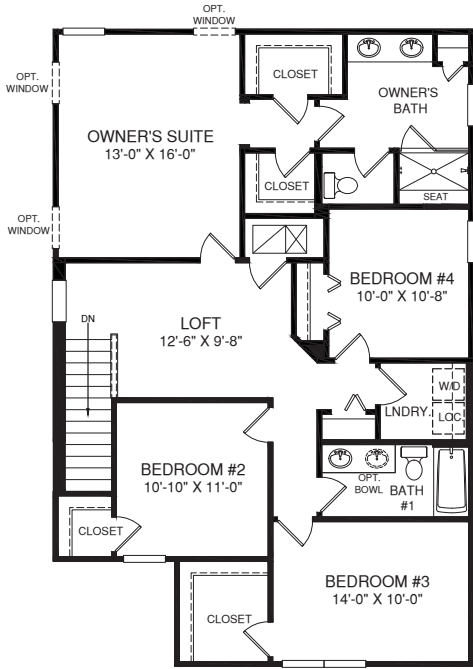
UPPER LEVEL
