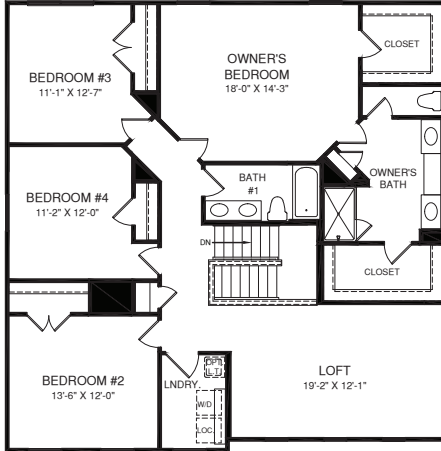
UPPER LEVEL
