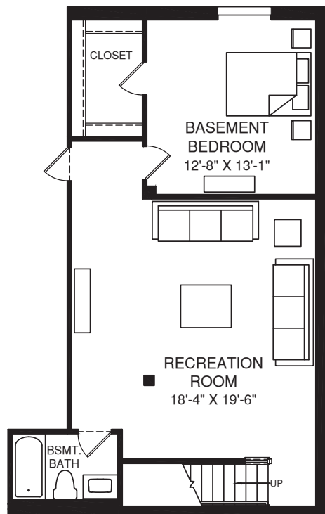
OPT. BASEMENT BEDROOM
