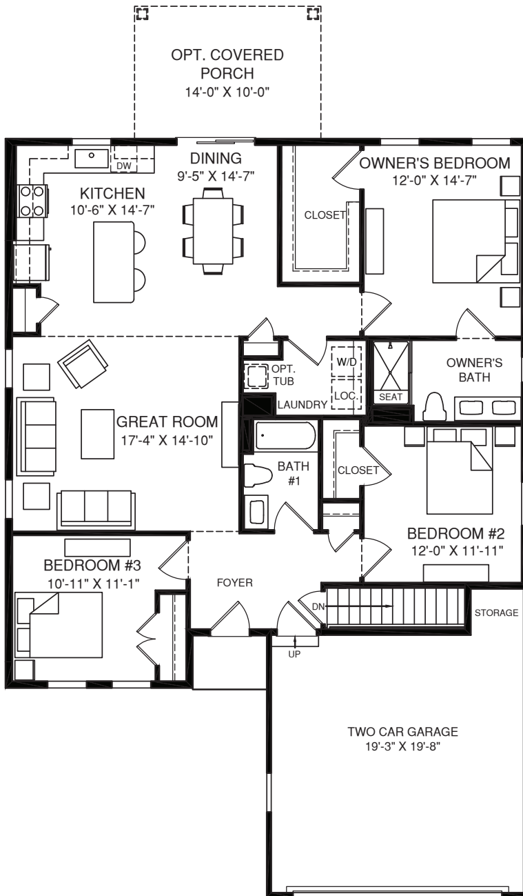
MAIN LEVEL
