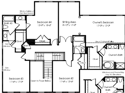
Second Floor w/ 4 Bedrooms, Sitting Area & 3 Baths Available Only w/ Opt. 4 Ext. @ Family Room
