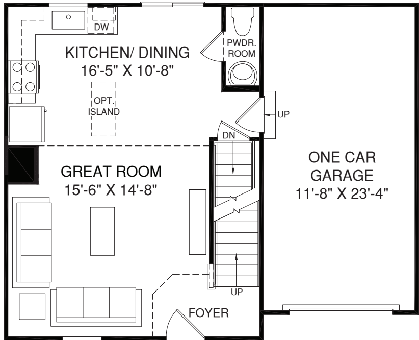
MAIN LEVEL
