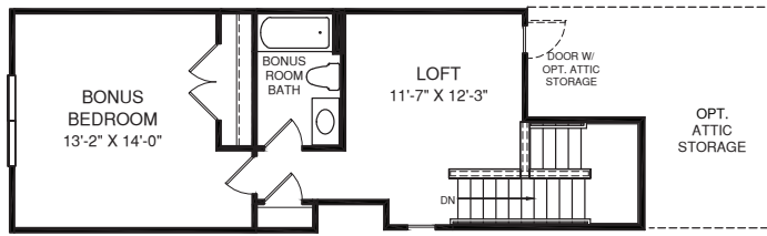
OPT. BONUS BEDROOM W/ LOFT
