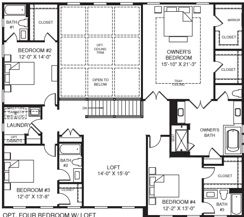
OPT. FOUR BEDROOM W/ LOFT
