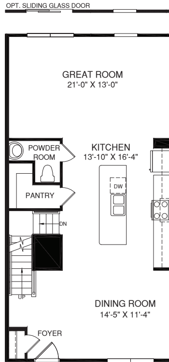
MAIN LEVEL
