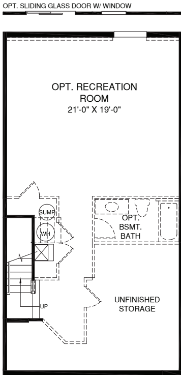
LOWER LEVEL
