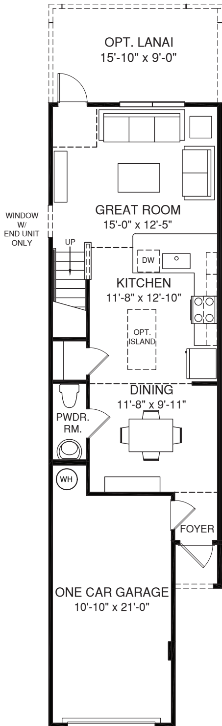
MAIN LEVEL
