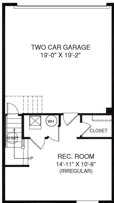
LOWER LEVEL
