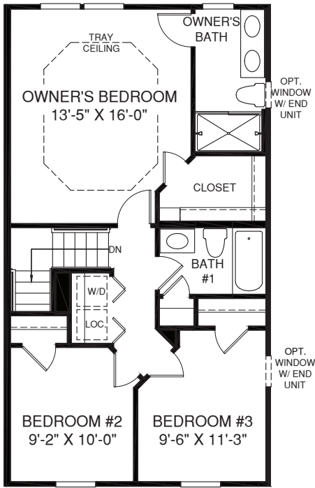
UPPER LEVEL
