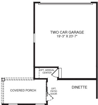
OPT. REAR ATTACHED GARAGE W/ OPT. EXPANDED REAR COVERED PORCH
