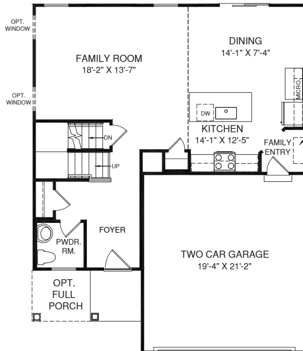
MAIN LEVEL
