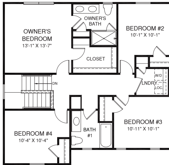
UPPER LEVEL
