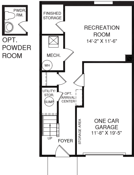
LOWER LEVEL
