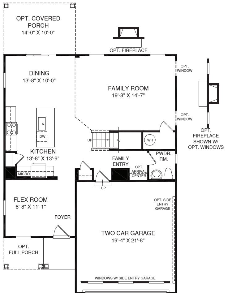
MAIN LEVEL
