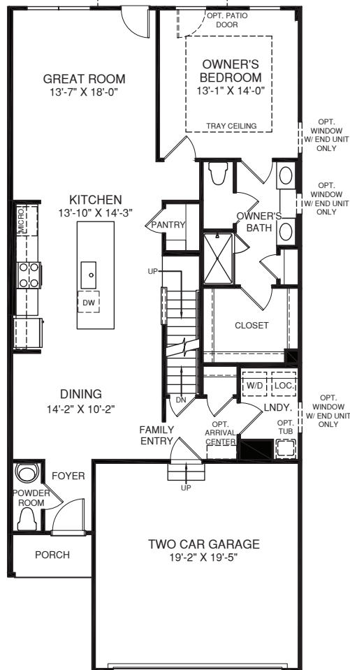
MAIN LEVEL
