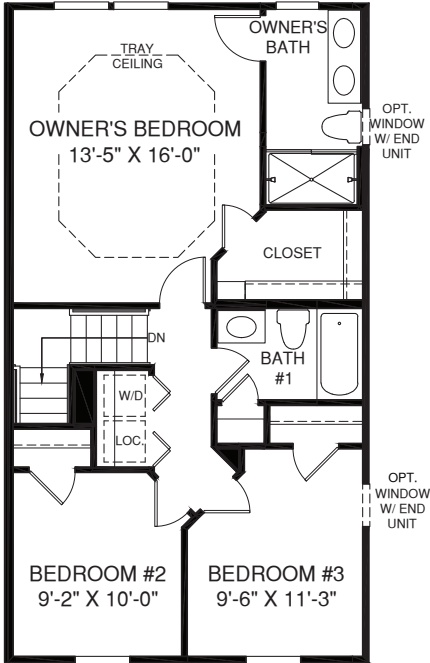
UPPER LEVEL
