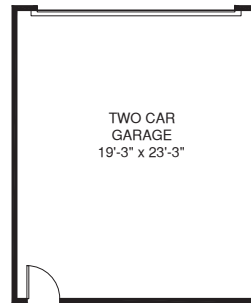
DETACHED GARAGE
