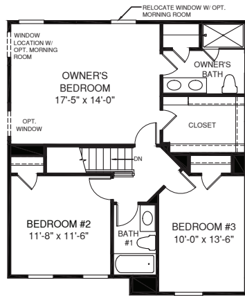
OPT. OWNER'S BATH W/ SOAKING TUB & SHOWER
