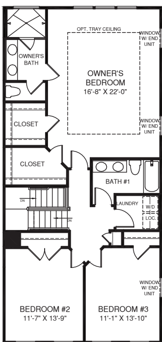
UPPER LEVEL
