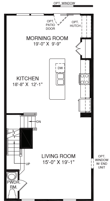
MAIN LEVEL
