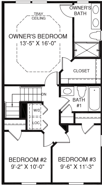
UPPER LEVEL
