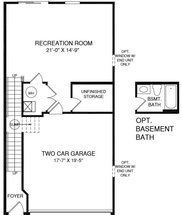
LOWER LEVEL
