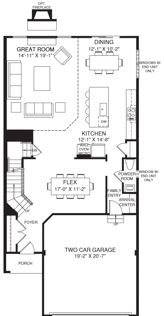
MAIN LEVEL
